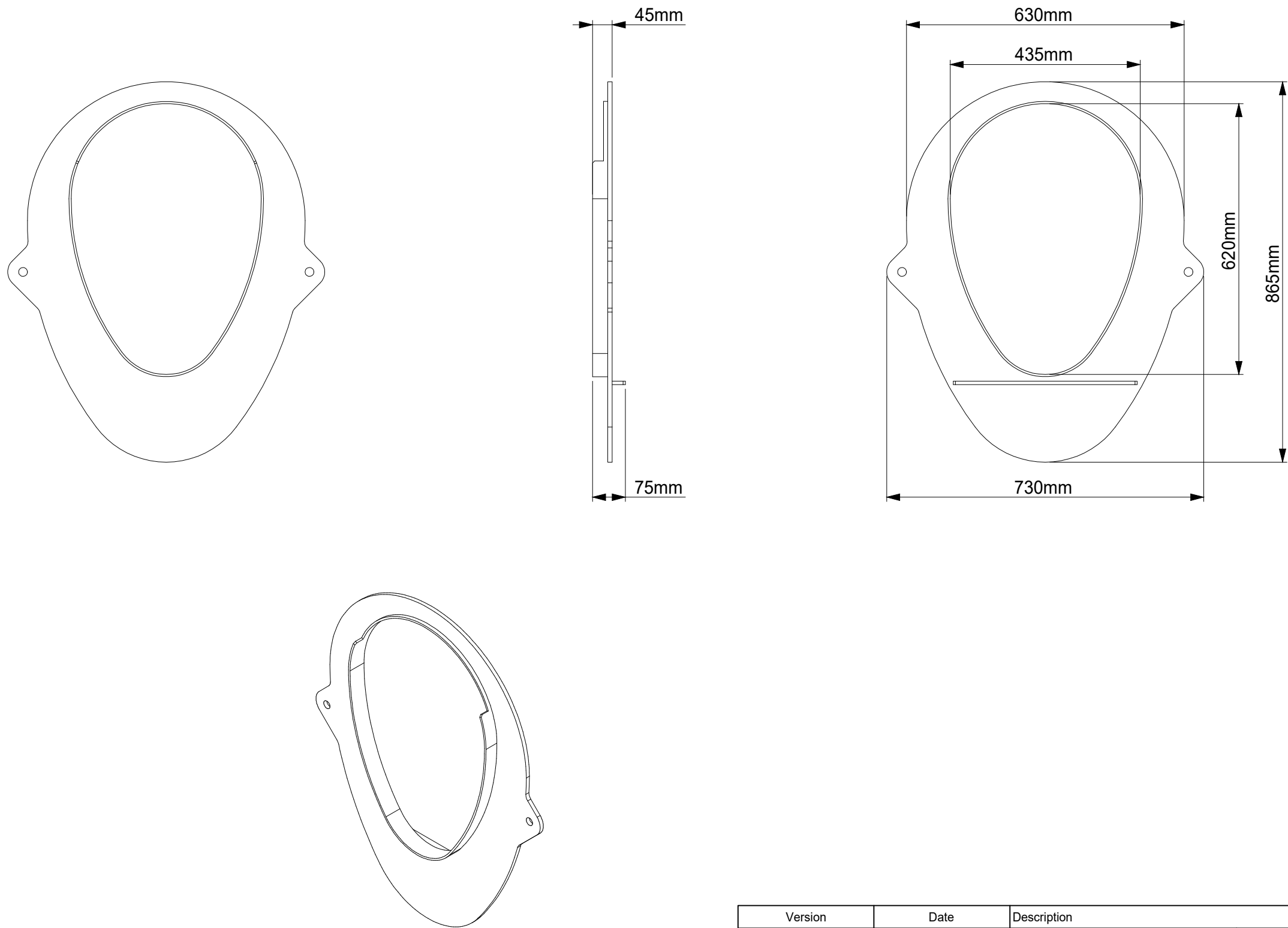
ISOMETRIC VIEW
