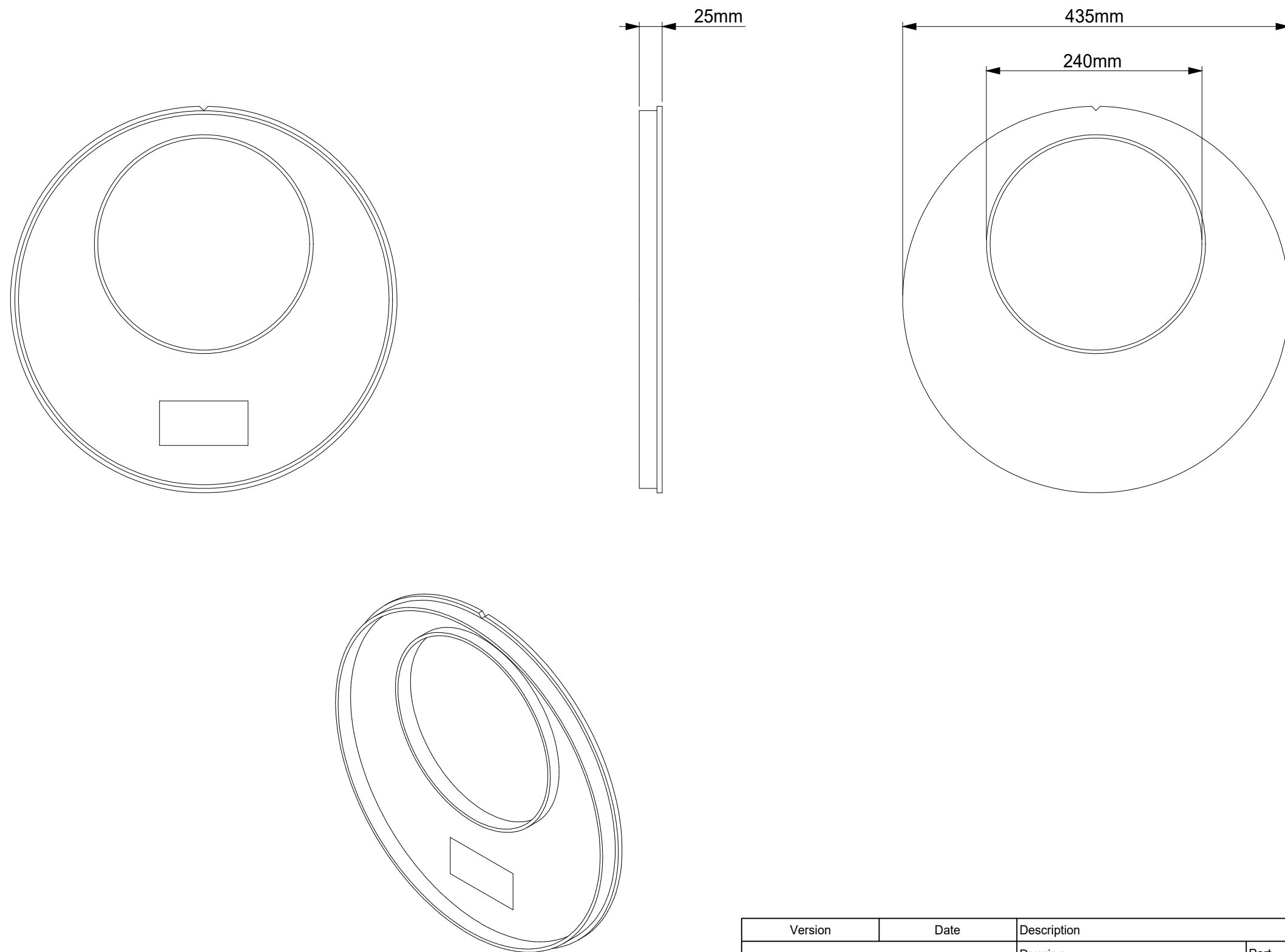
ISOMTERIC VIEW
