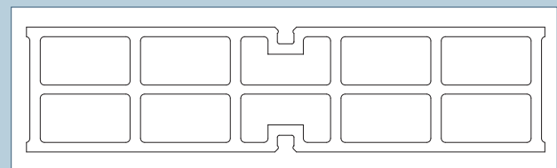
Template of the grate of nominal width 100 (500 x 123 mm)
