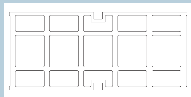
Template of the grate of nominal width 200 (500 x 223 mm)
