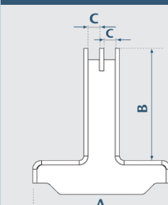
TWIN – central
