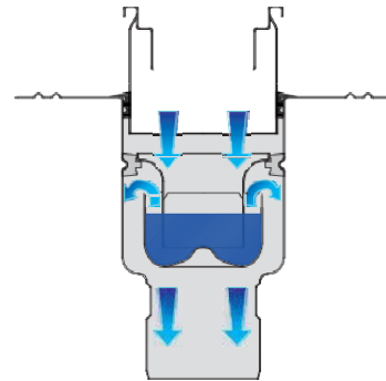
Discreet Channel Vertical Outlet
