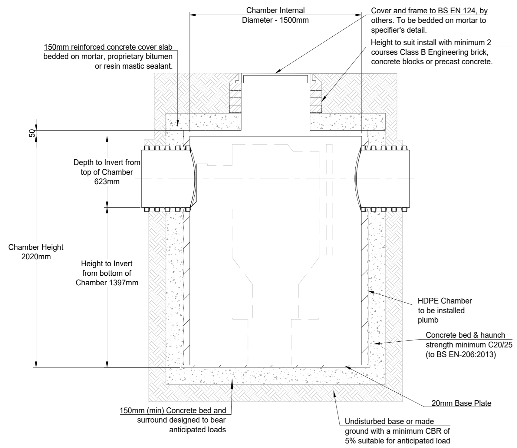
Section View of Stormsed Vortex 1500
