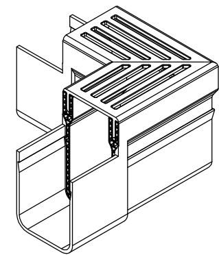
19006 THRESHOLD DRAIN CORNER UNIT - SILVER GRATING
