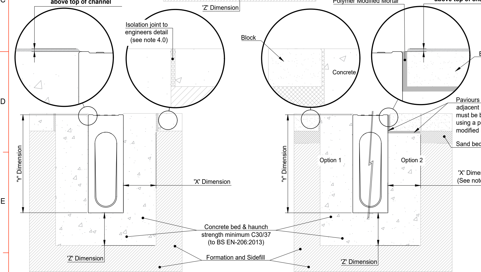
1 : 10 ACO RoadDrain Concrete Pavement
