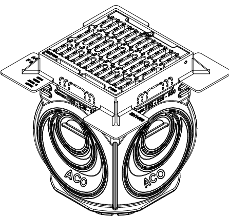
ISOMETRIC VIEW ACCESS CHAMBER
