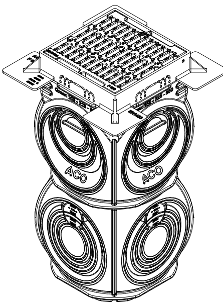
ISOMETRIC VIEW OUTLET/INLET CHAMBER
