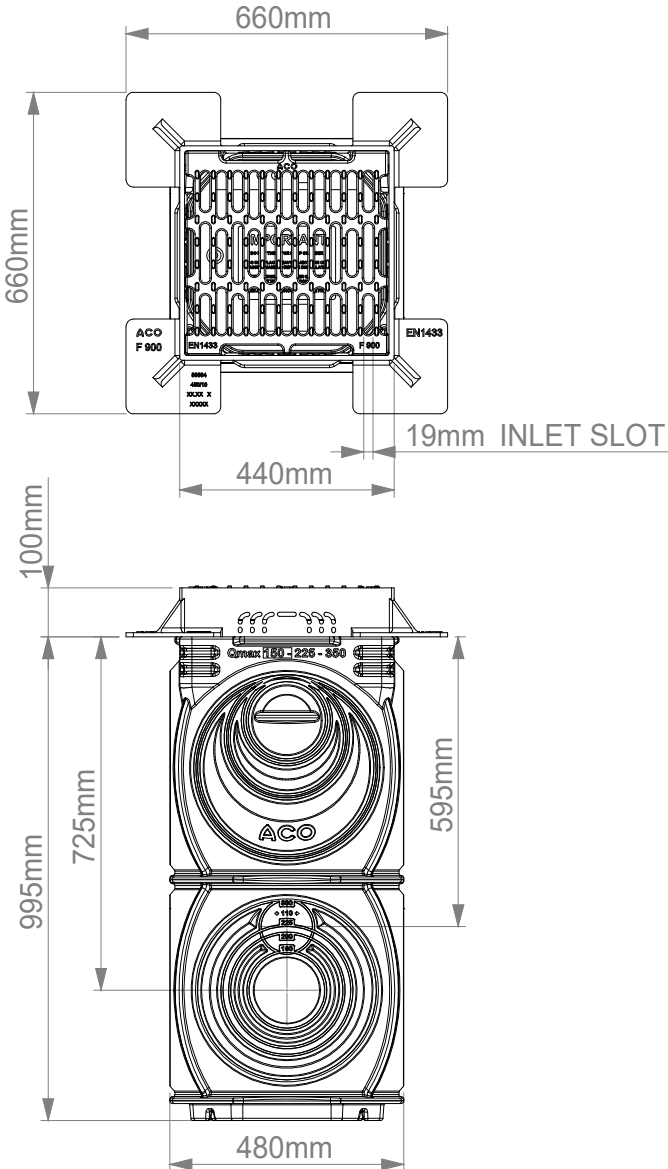
32973 - OUTLET/INLET CHAMBER WITH F900 SLOTTED COVER AND FRAME
