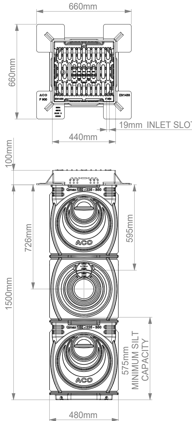
32975 - OUTLET/INLET CHAMBER WITH F900 SLOTTED COVER AND FRAME
