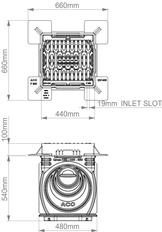
32971 - ACCESS CHAMBER WITH F900 SLOTTED COVER AND FRAME
