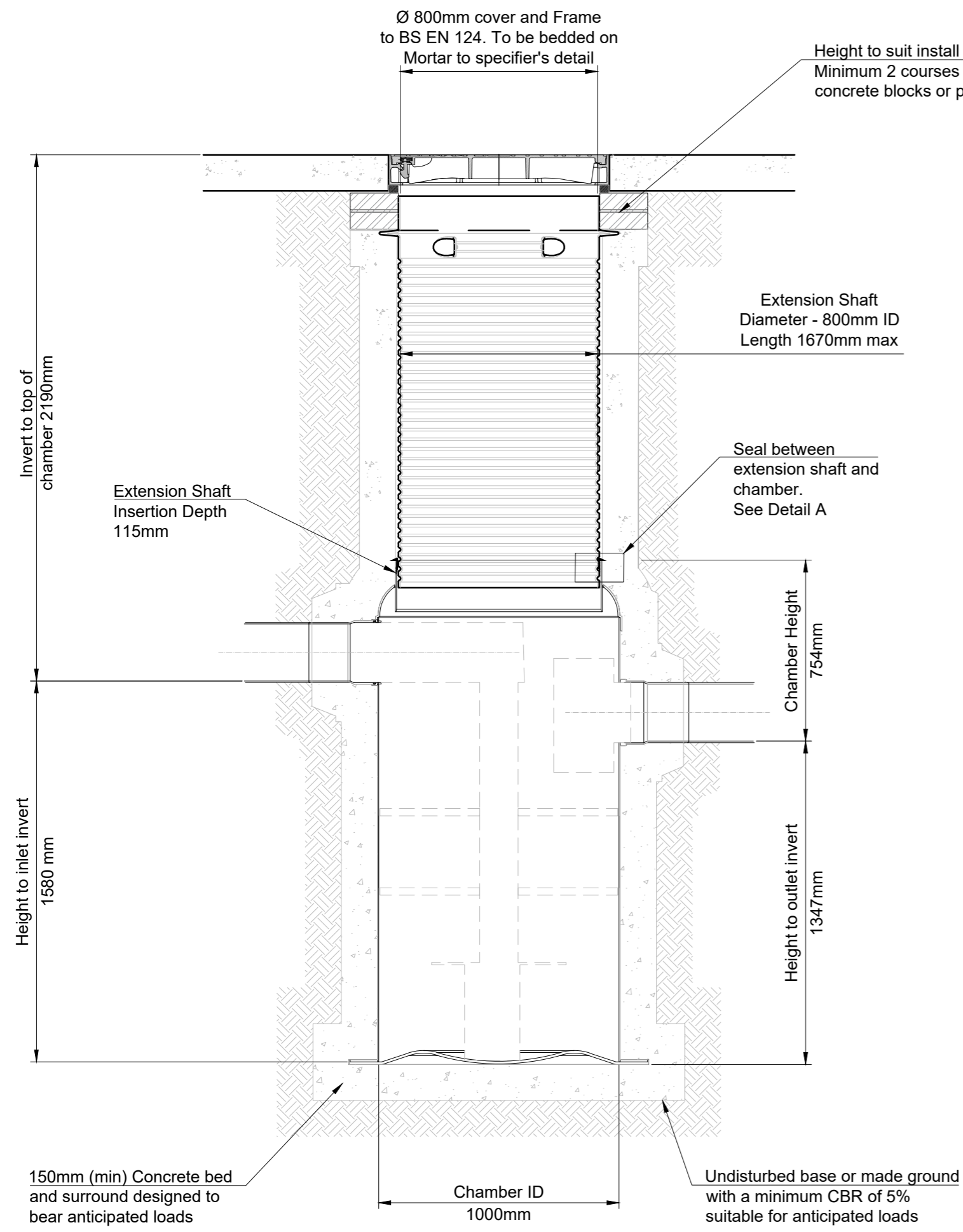
Section View of StormSed Filter 1000
