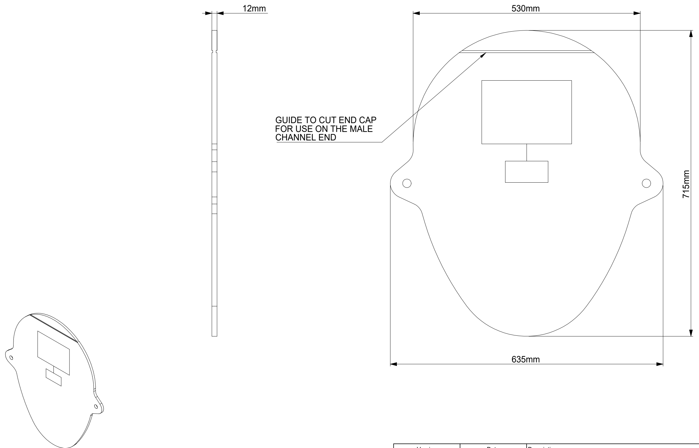
ISOMETRIC VIEW SCALE 1:10
